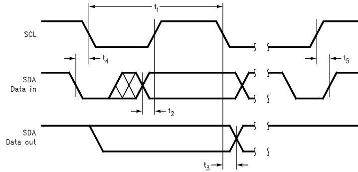
Figure 37. I²C Timing Diagram
